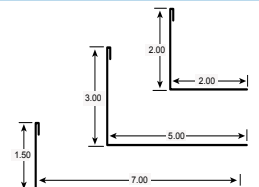
13. Angle Trim
