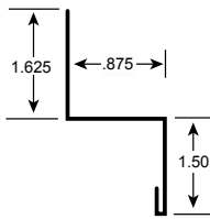
2. "Z" Strip
