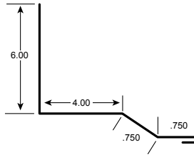
8. Wall Flashing
