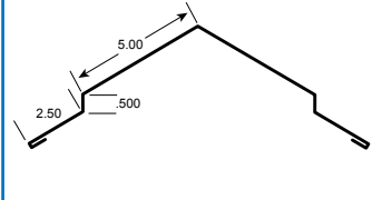
10. Ridge Cap
