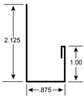
1. "J" Channel
