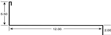
11. 1-Piece Soffit
