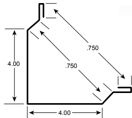
15. Outside Corner
