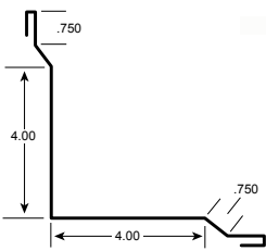
14. Inside Corner
