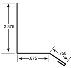
6. Drip Flashing
